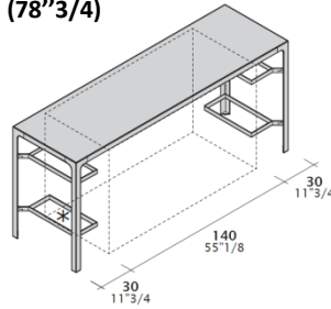
W 200 counter (78"3/4)
